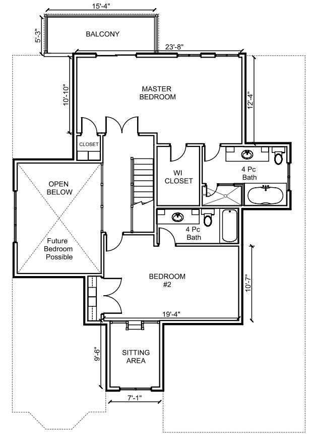
Second Floor 1,015 sf
