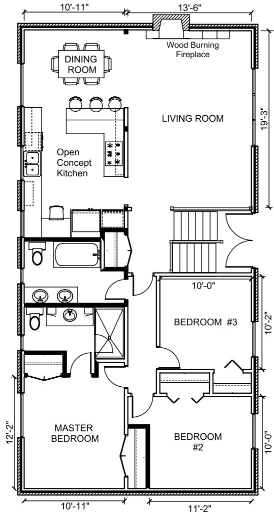
MAIN LEVEL - Concept A
