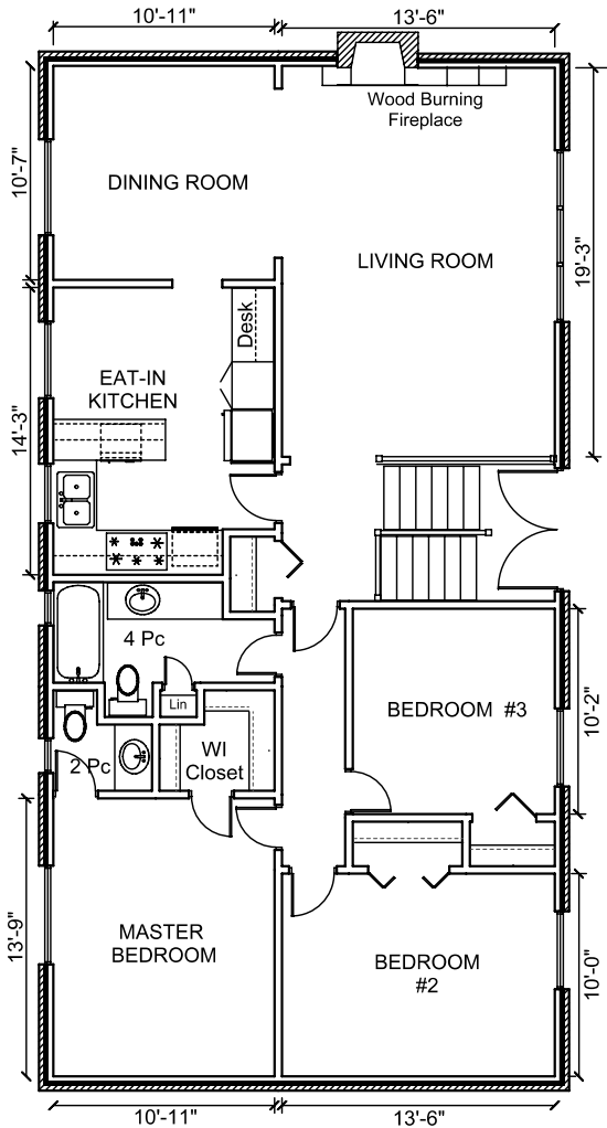
MAIN LEVEL - EXISTING LAYOUT
