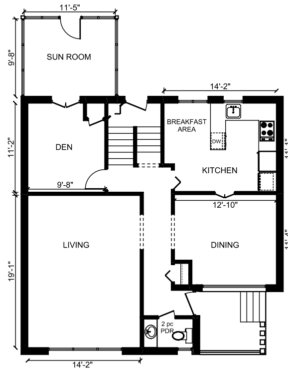
MAIN FLOOR
