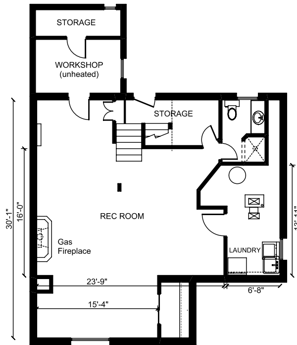
BASEMENT
